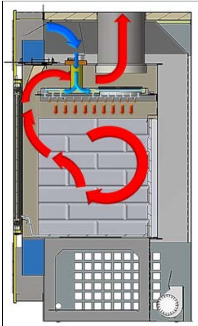
Figure 3-3: Air Flow through Secondary Air Channel
