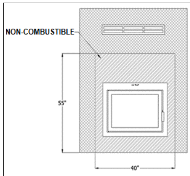
Figure 3-39: Front Chase for Clean face Linear Louver Configuration
