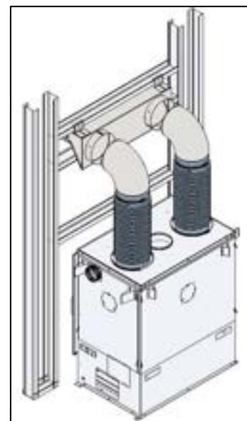
Figure 3-30: CAC8 Duct Installation
