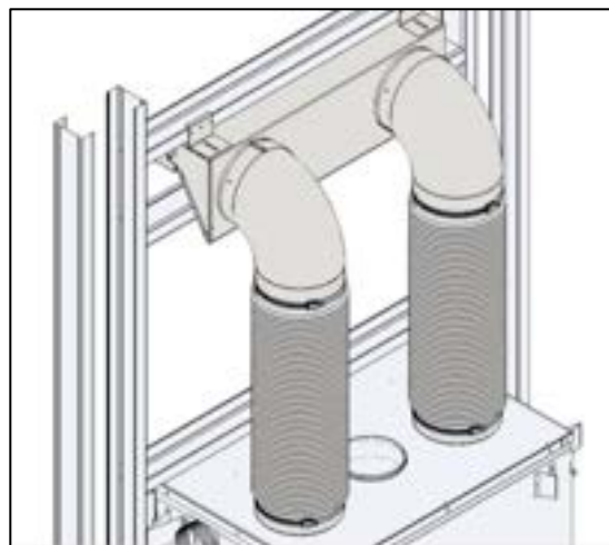
Figure 3-32: The Two Bottom Worm Gear Clamps Tightened
