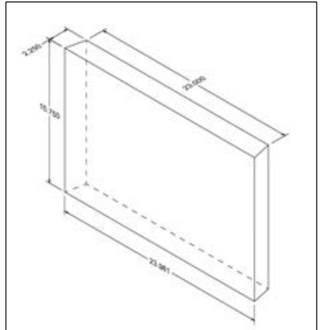
Figure 4-2: 32SF Non-Usable Firebox
