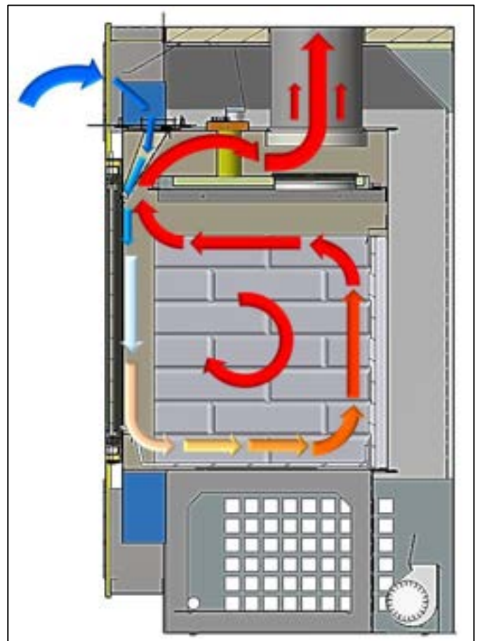
Figure 3-2: Air Flow through Primary Air Booster Channel
