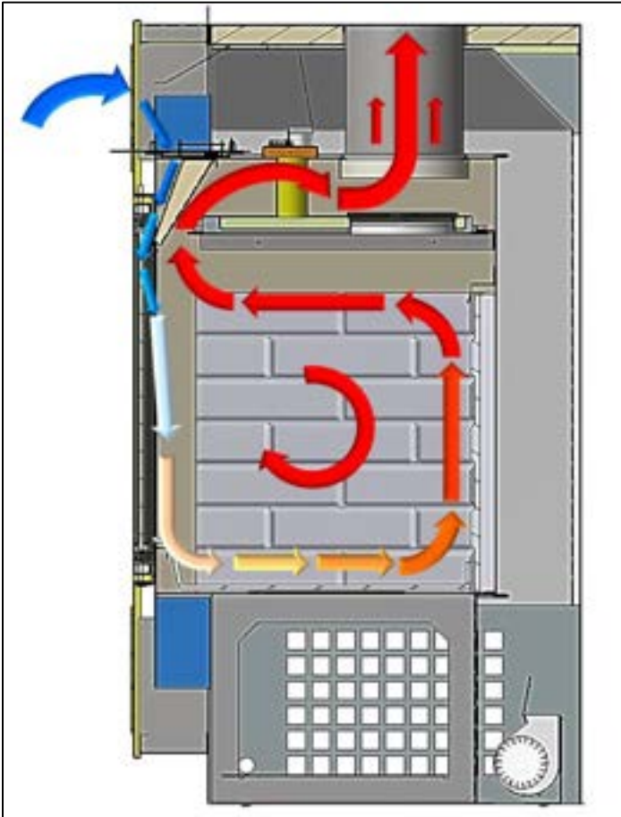
Figure 3-1: Air Flow through Primary Air Wash Channel
