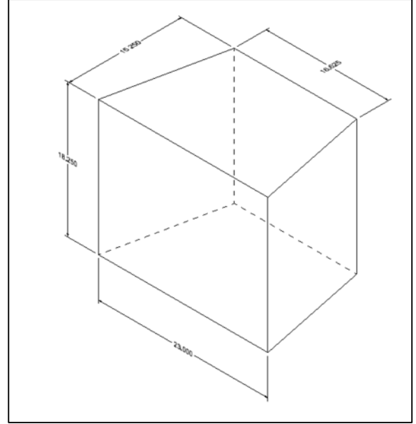
Figure 4-1: 32SF Usable Firebox
