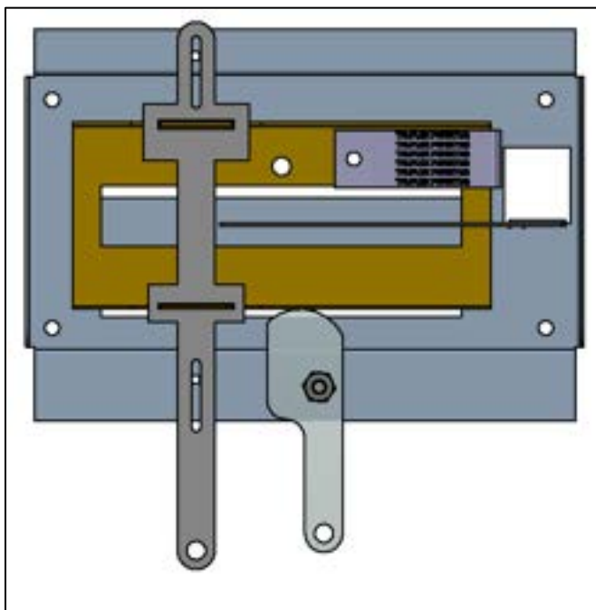
Figure 17-1: PAC Set to Maximum Burn Rate Position
