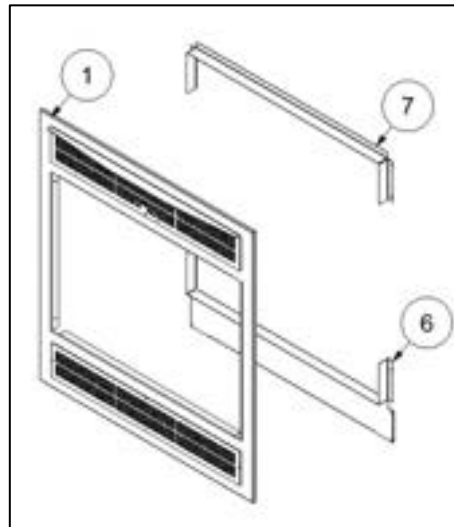
Figure 3-14: Traditional Surround Components
