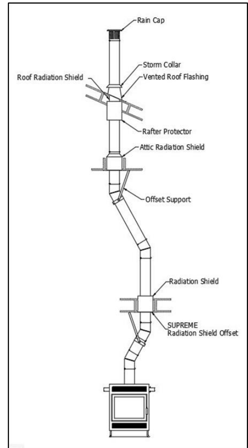
Figure 3-7: Offset Installation
