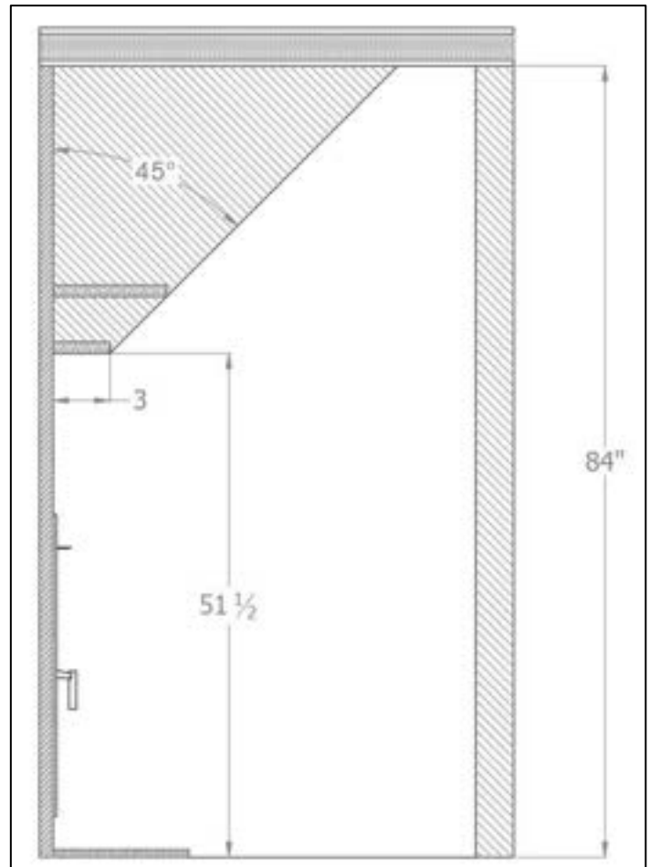
Figure 3-40: Mantle Clearance
