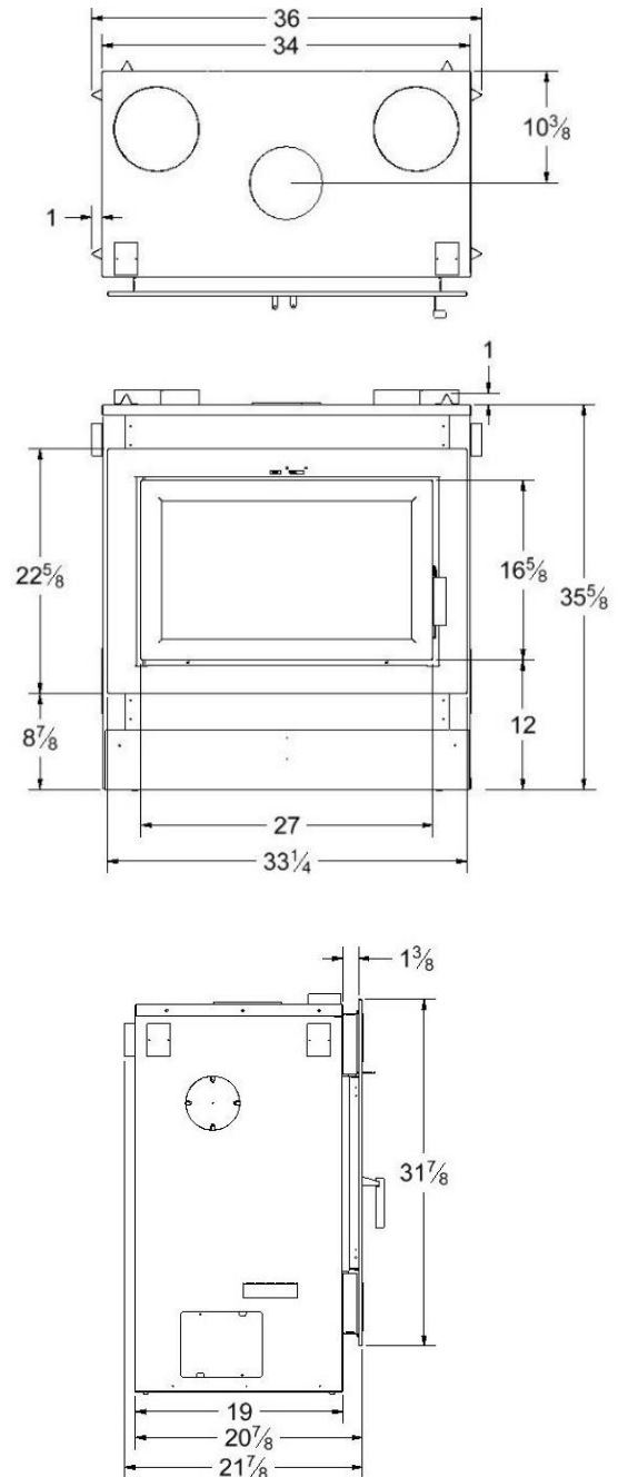
Figure 2-2: Astra 24 Clean Face Dimensions
