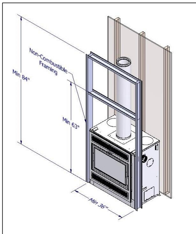
Figure 3-17: Minimum Astra 24 Framing Dimensions
