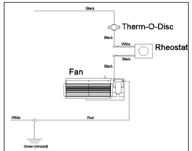
Figure 3-24: Electrical Diagram
