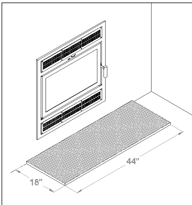
Figure 3-18: Hearth Extension
