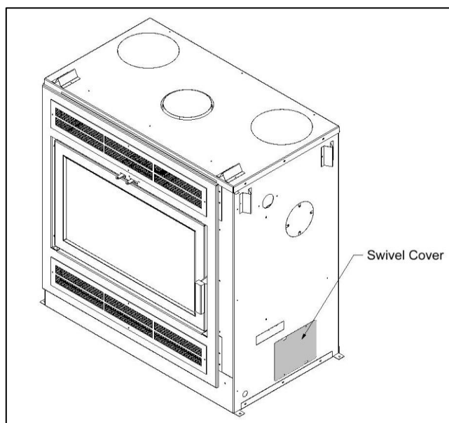
Figure 3-9: Intake Swivel Cover Closed
