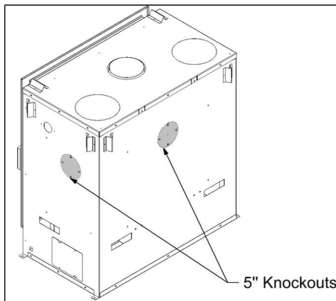
Figure 4-2: Front Cover Installation for Traditional Face
