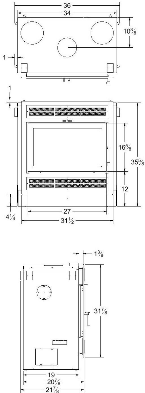
Figure 2-1: Astra 24 Traditional Dimensions
