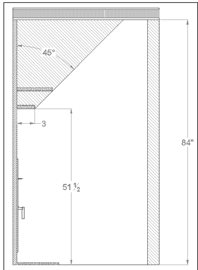
Figure 3-22: Mantel Clearances
