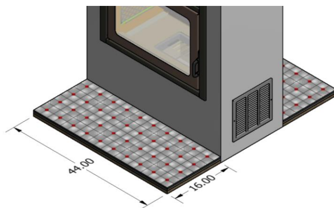
Figure 14 – Hearth extension
