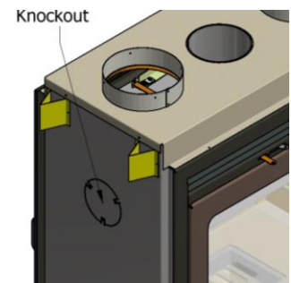
Figure 23 – Knockout
