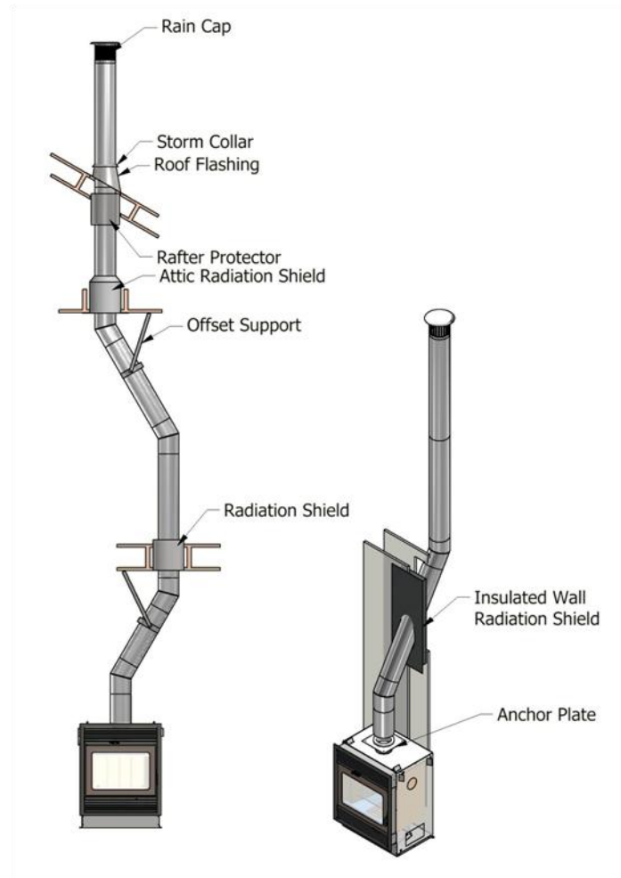
Figure 25 – Chimney Installation
