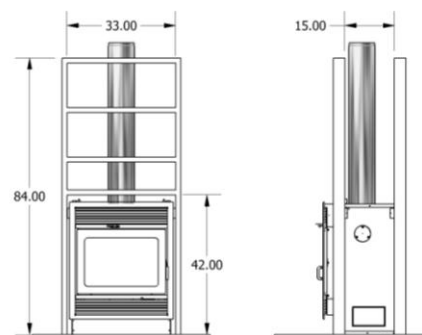
Figure 16 – Framing
