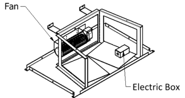
Figure 22 – Fan Kit
