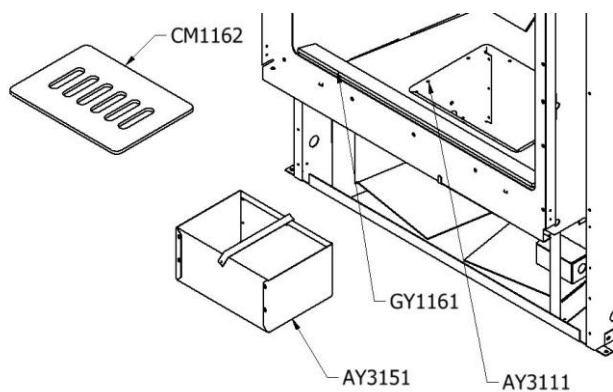
Figure 23 – Fan Access
