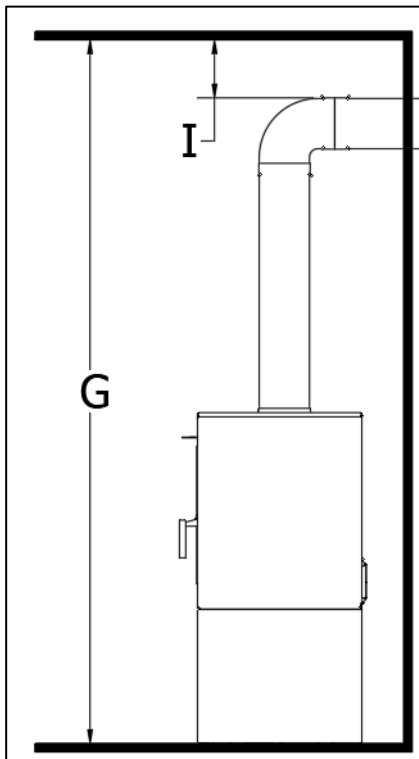
Figure 3-3: Clearances to Combustibles Through Wall Installation
